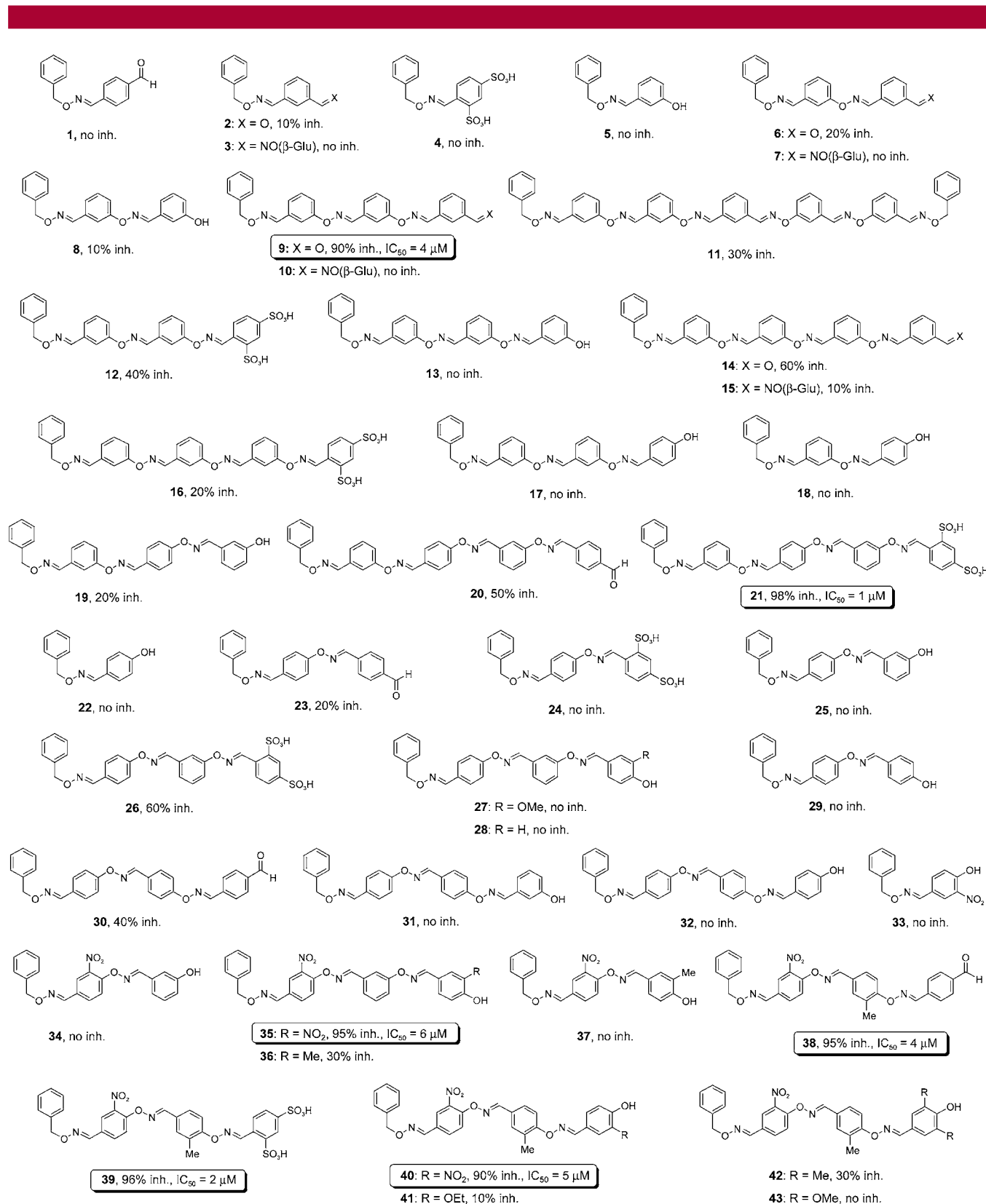
Figure 3. Oxime oligomers tested for inhibition. Inhibition data of proteolytic activity for \alpha -chymotrypsin in the presence of 10 \mu M inhibitor are given for each oligomer as well as IC_{50} values of compounds with more than 90% inhibition.
